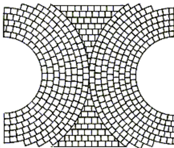
CIRCULAR AND RUNNING BOND
